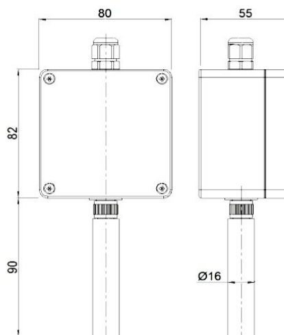
Sensor probe HT-RP16
