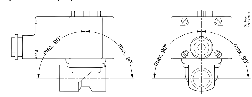
Figure 9: Mounting angle
